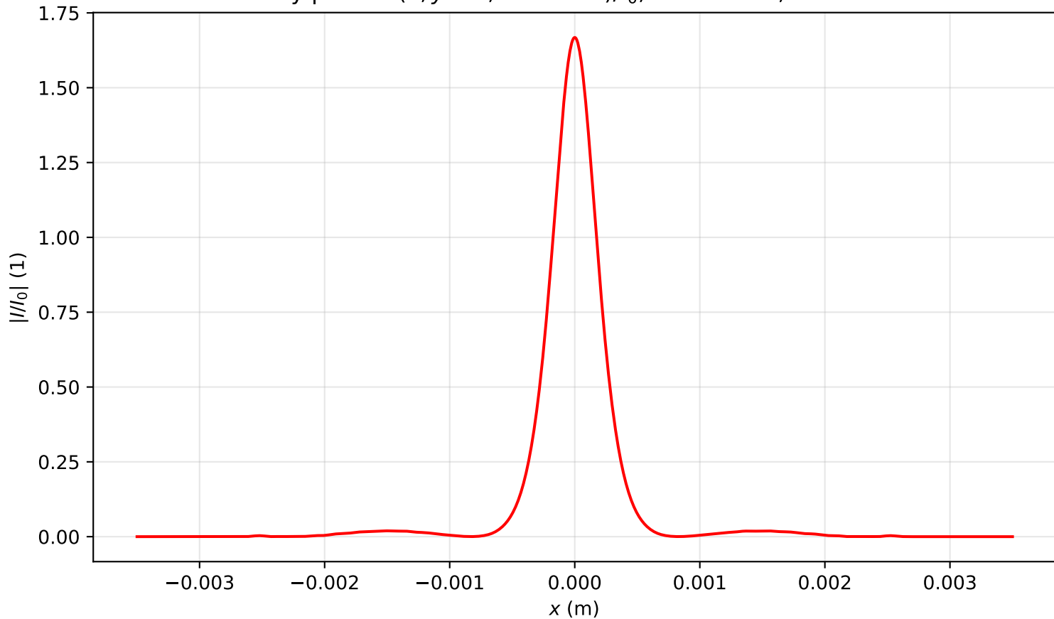
Intensity profile I(x, y = 0, z = 1.115)/I_0 , P_{in}=1.0P_{cr} , artificial time
